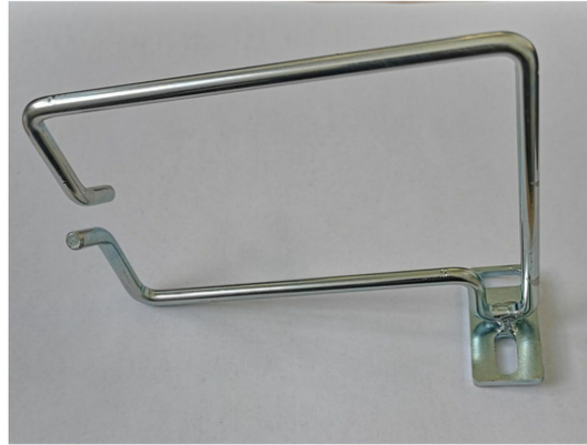
Shunting bracket for side mounting in rack, 80x120mm
