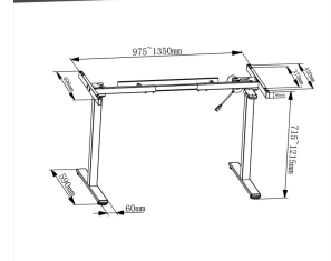
DA-90452 Electrically Height-Adjustable Table Frame, Single Motor, 2 Levels, Gray
